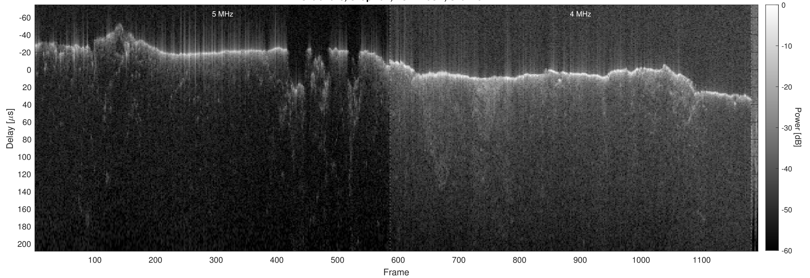
Orbit 4043, Chapman, No Window, Channel 2
