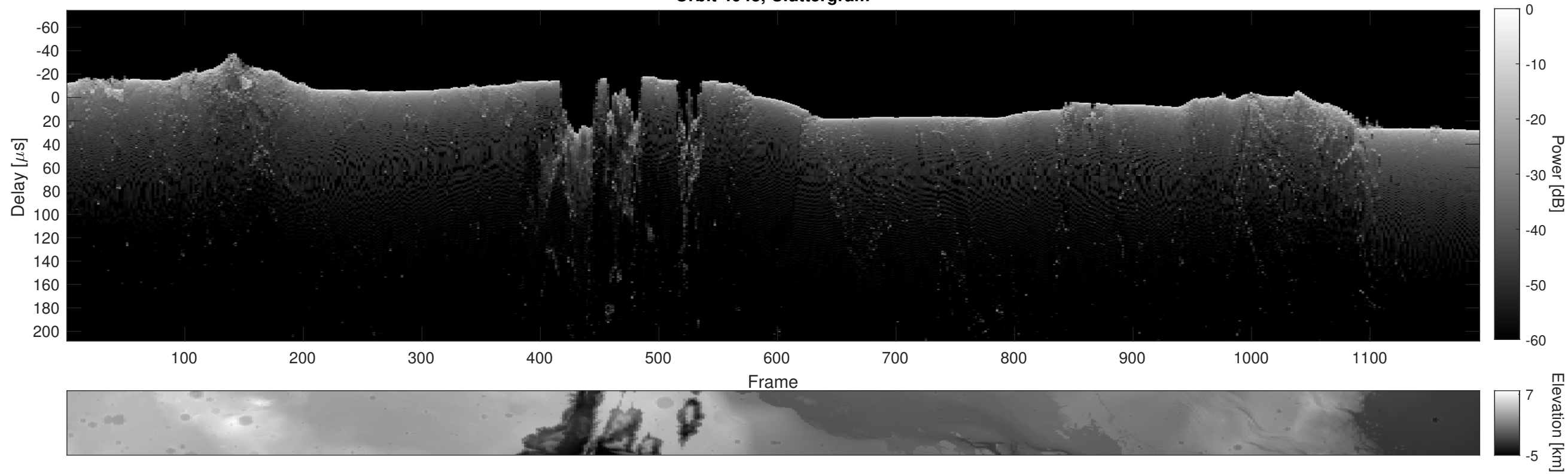
Orbit 4043, Cluttergram
