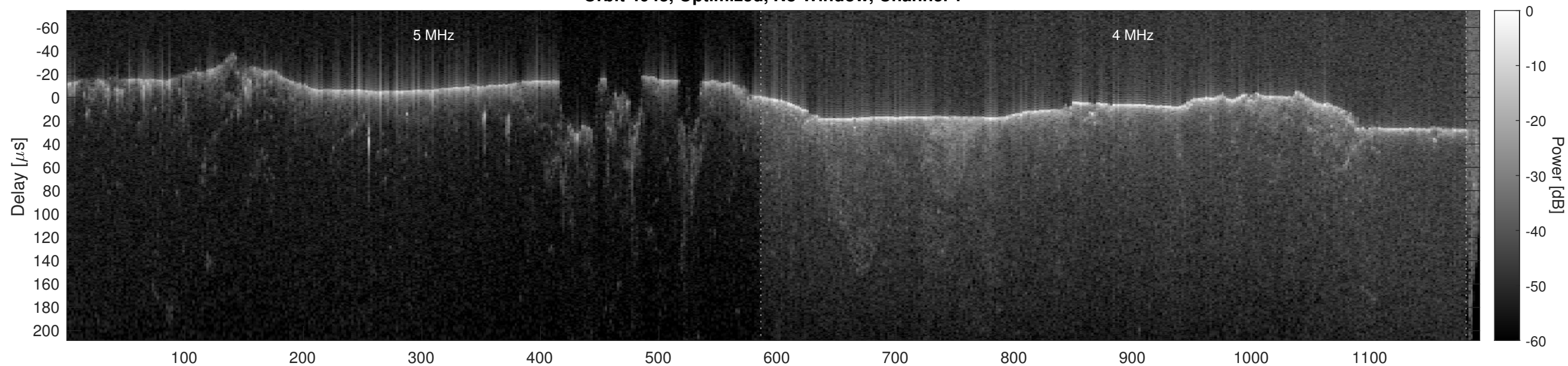
Orbit 4043, Optimized, No Window, Channel 2
