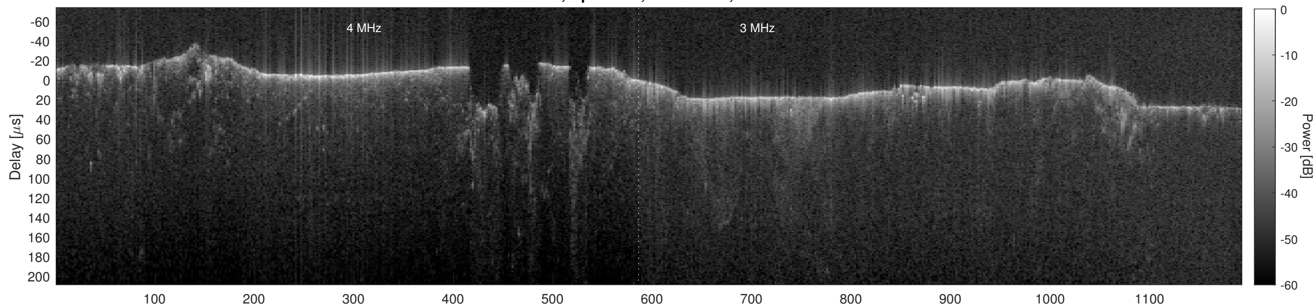
Orbit 4043, Cluttergram
