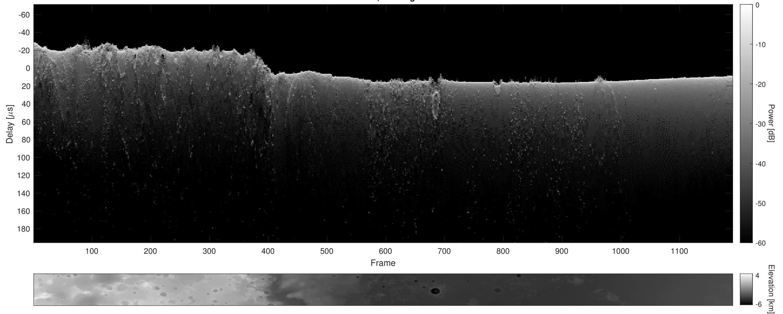
Orbit 4044, Cluttergram
