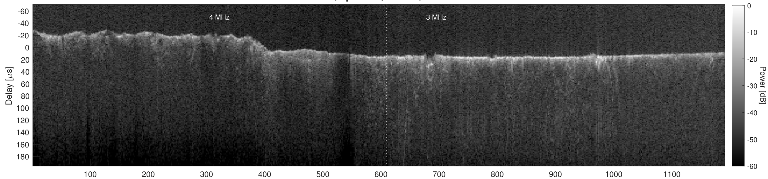
Orbit 4044, Cluttergram
