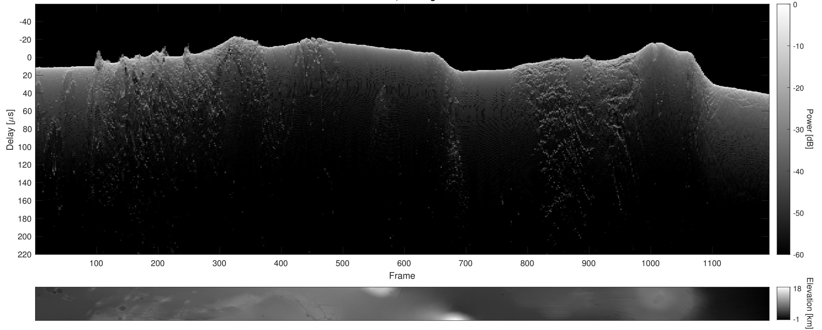
Orbit 4047, Cluttergram
