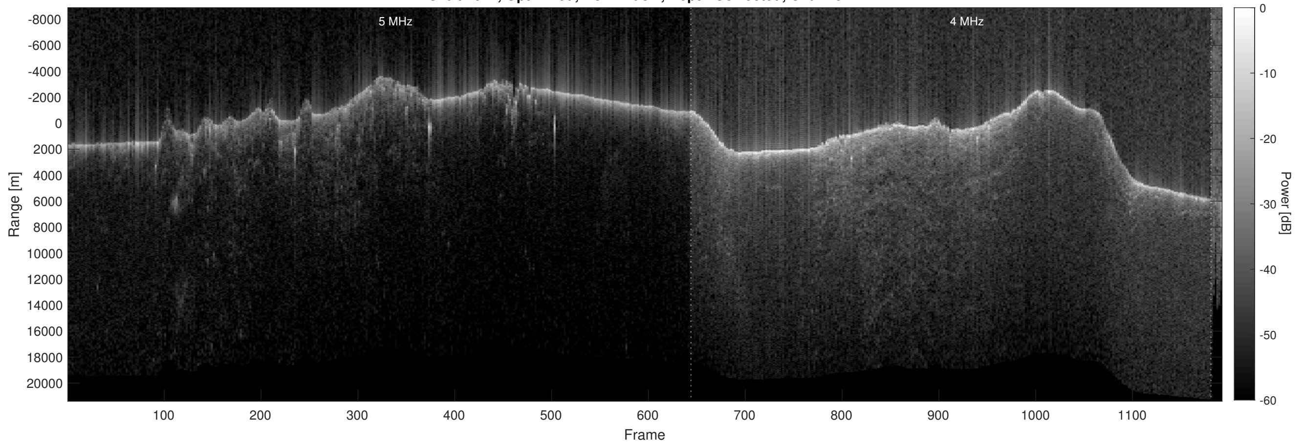
Orbit 4047, Optimized, No Window, Depth-Corrected, Channel 2
