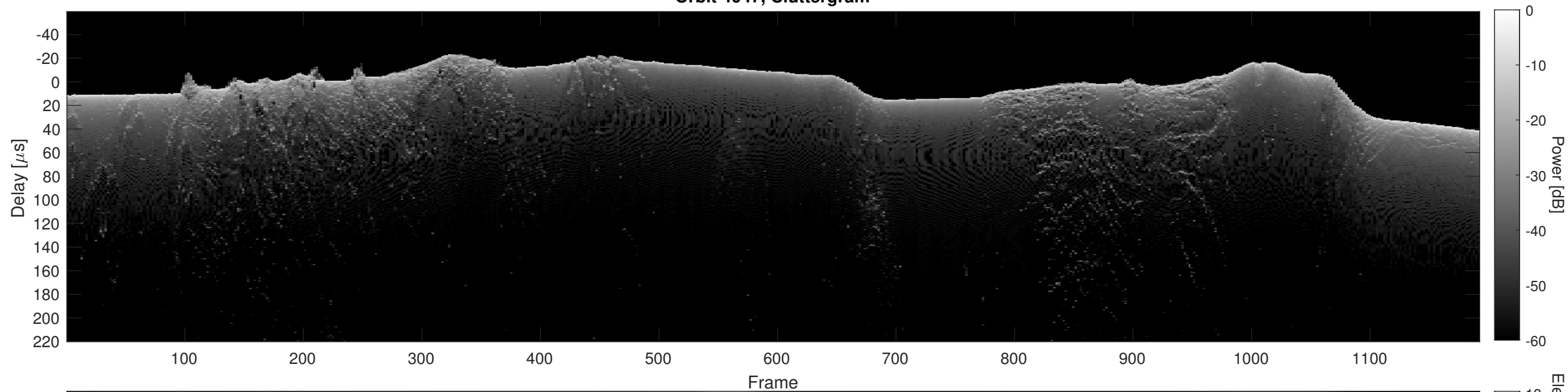
Orbit 4047, Cluttergram
