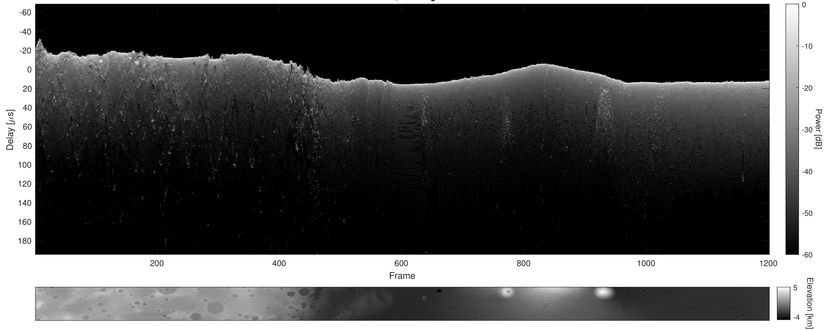
Orbit 4048, Cluttergram
