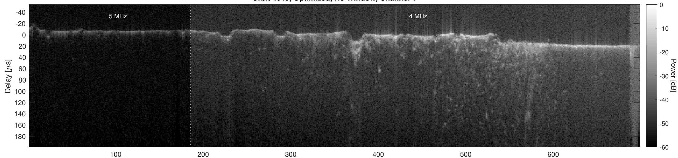
Orbit 4049, Optimized, No Window, Channel 2
