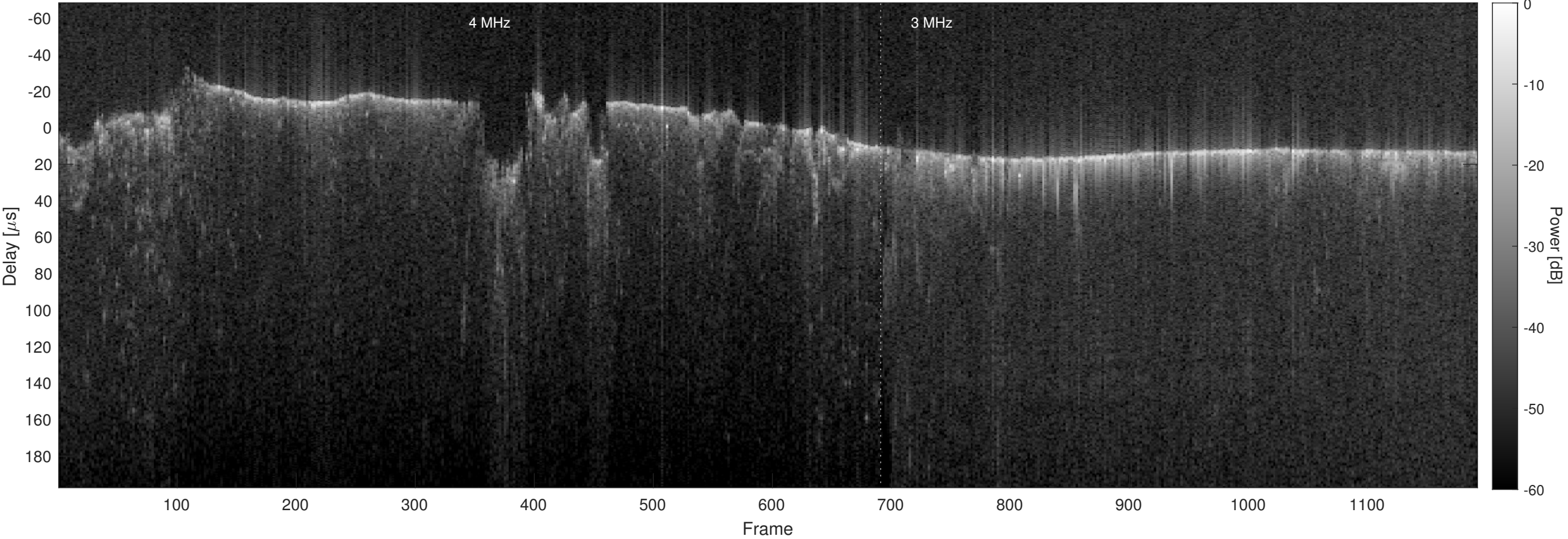
Orbit 4050, Optimized, No Window, Channel 2
