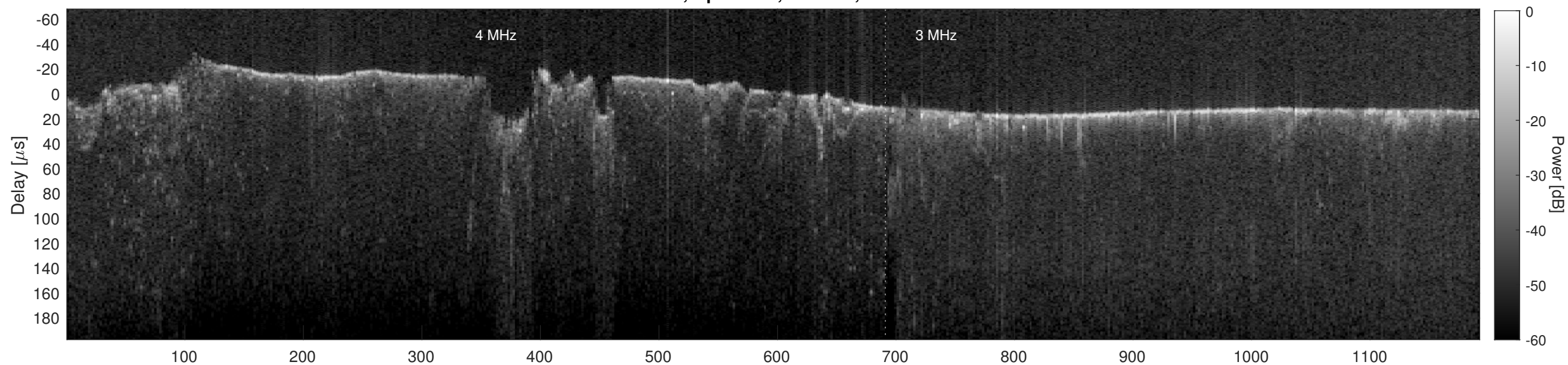
Orbit 4050, Cluttergram
