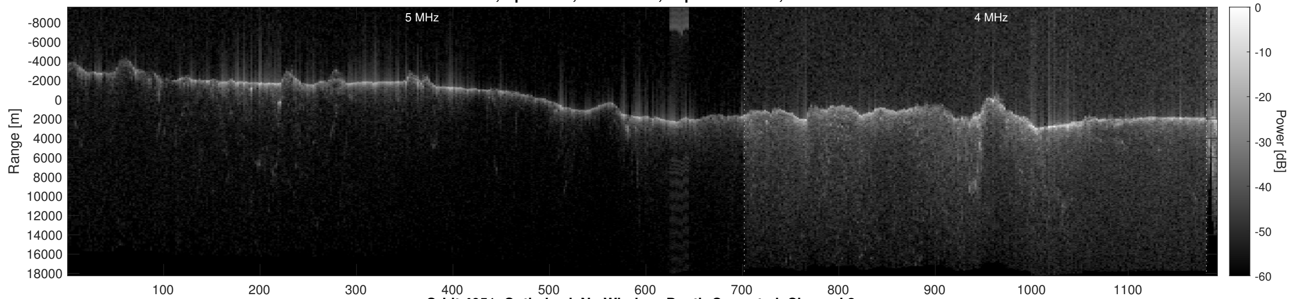
Orbit 4051, Optimized, No Window, Depth-Corrected, Channel 2
