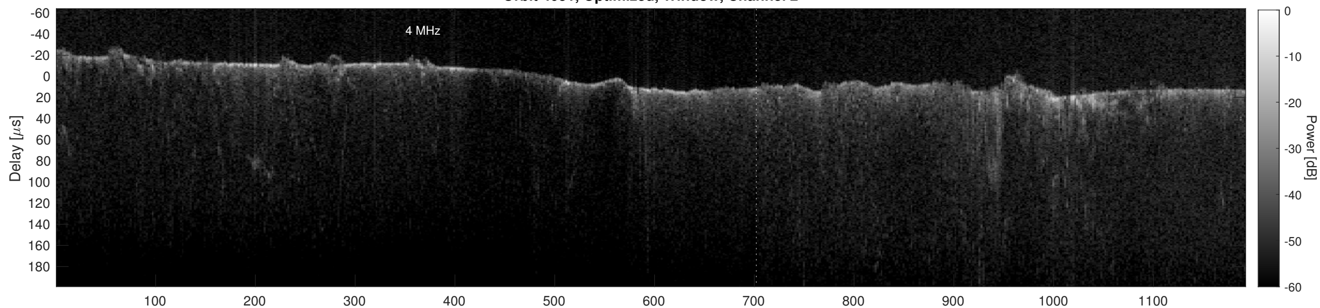
Orbit 4051, Cluttergram
