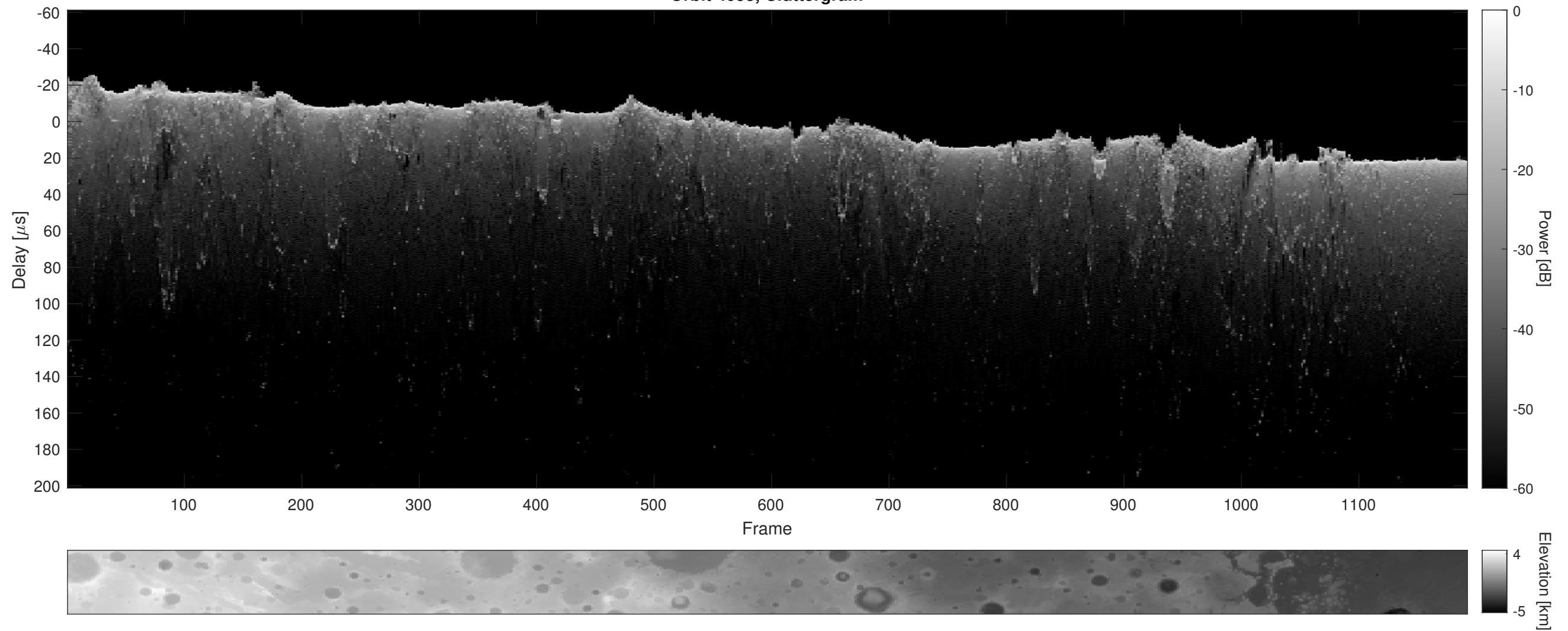
Orbit 4053, Cluttergram
