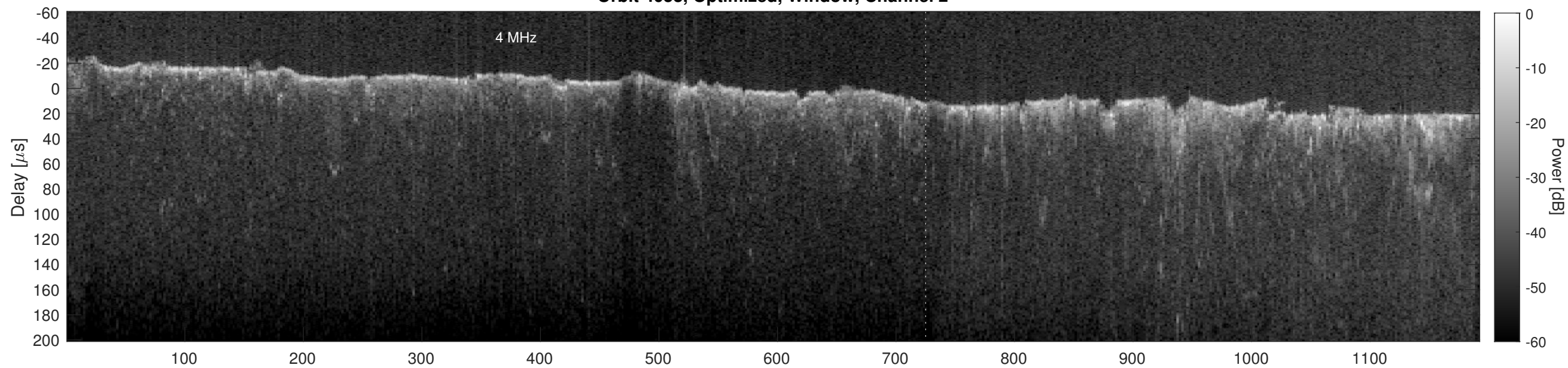
Orbit 4053, Cluttergram
