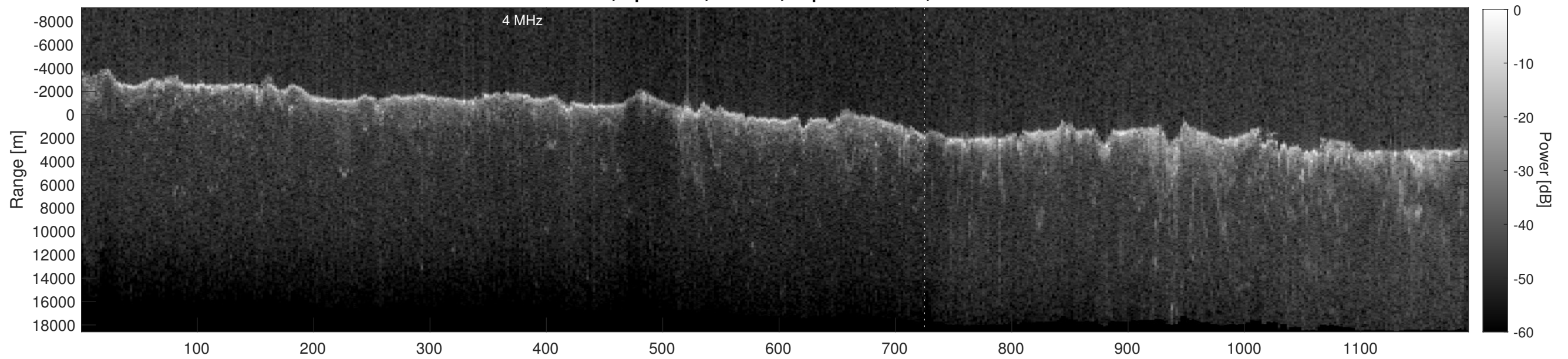
Orbit 4053, Depth-Corrected Cluttergram
