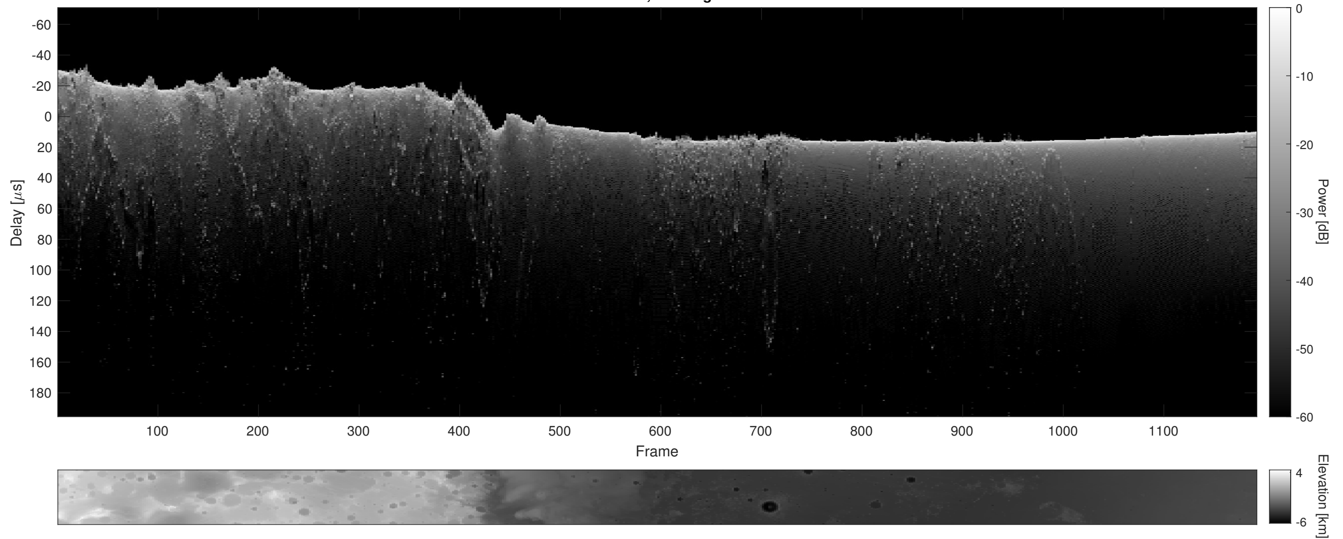
Orbit 4055, Cluttergram
