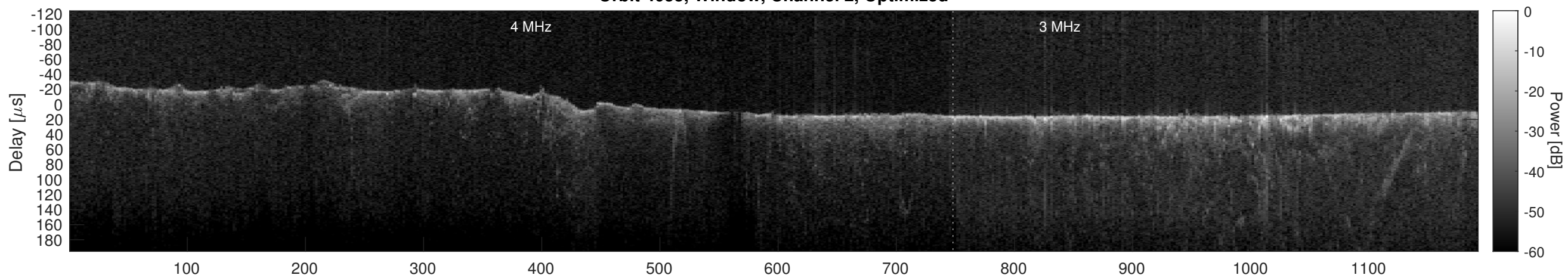
Orbit 4055, Cluttergram
