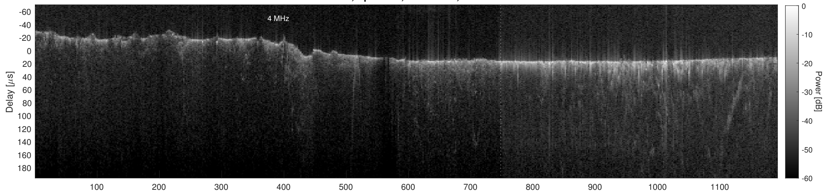
Orbit 4055, Cluttergram
