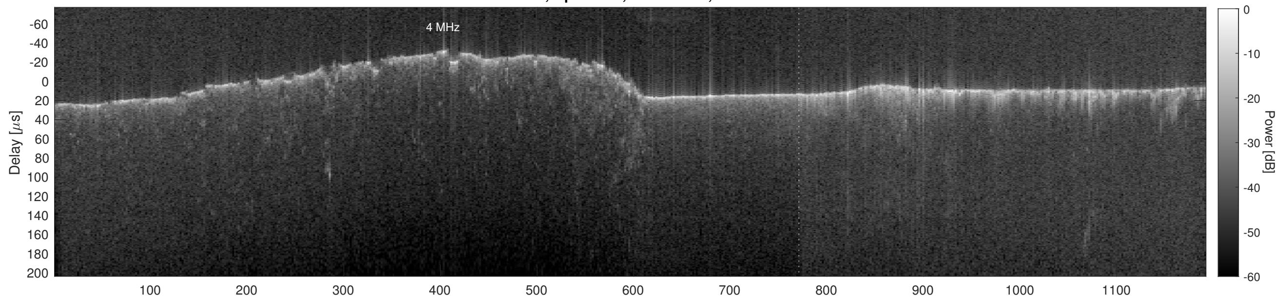
Orbit 4056, Cluttergram
