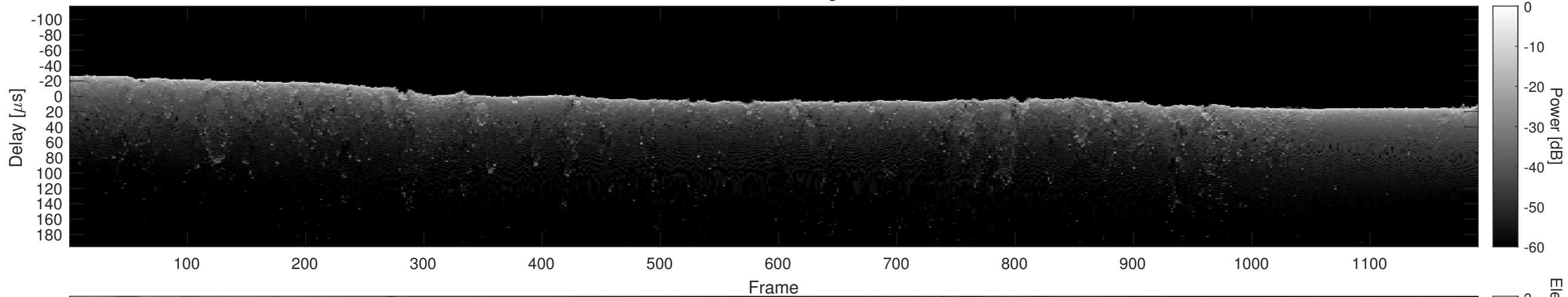
Orbit 4057, Cluttergram
