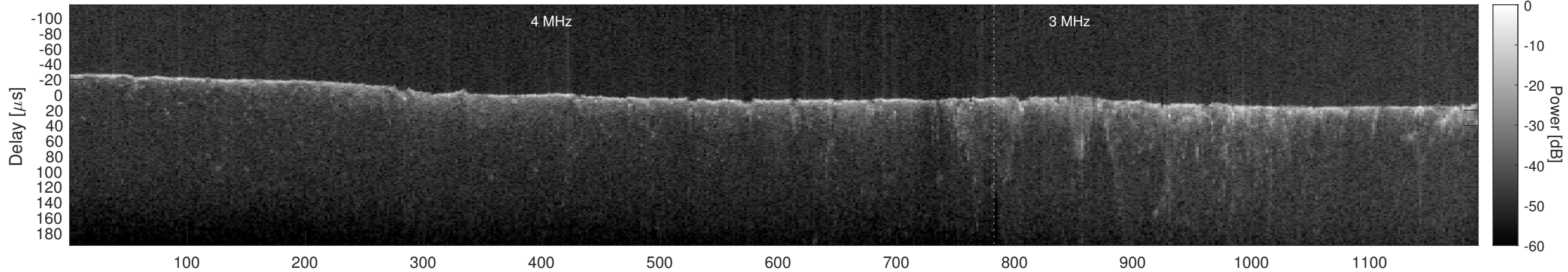
Orbit 4057, Cluttergram
