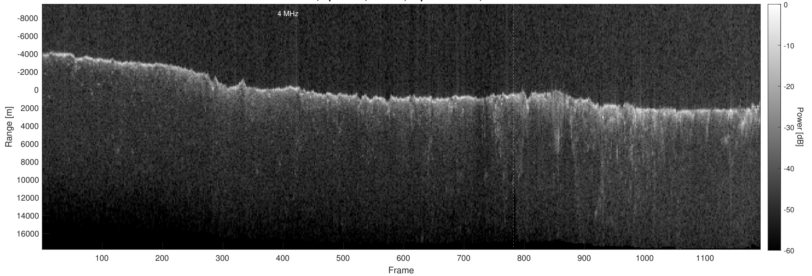
Orbit 4057, Optimized, Window, Depth-Corrected, Channel 2
