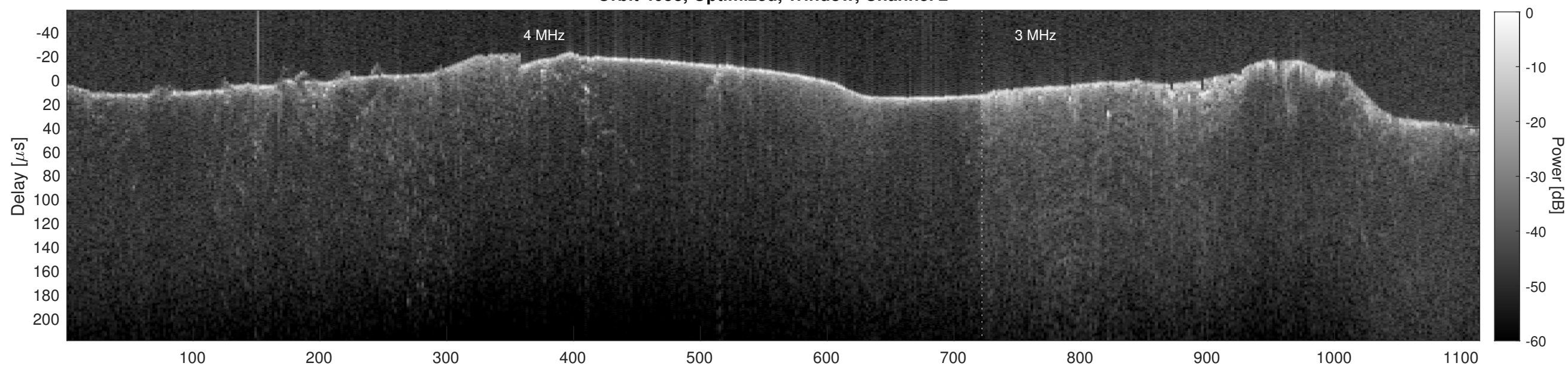
Orbit 4058, Cluttergram
