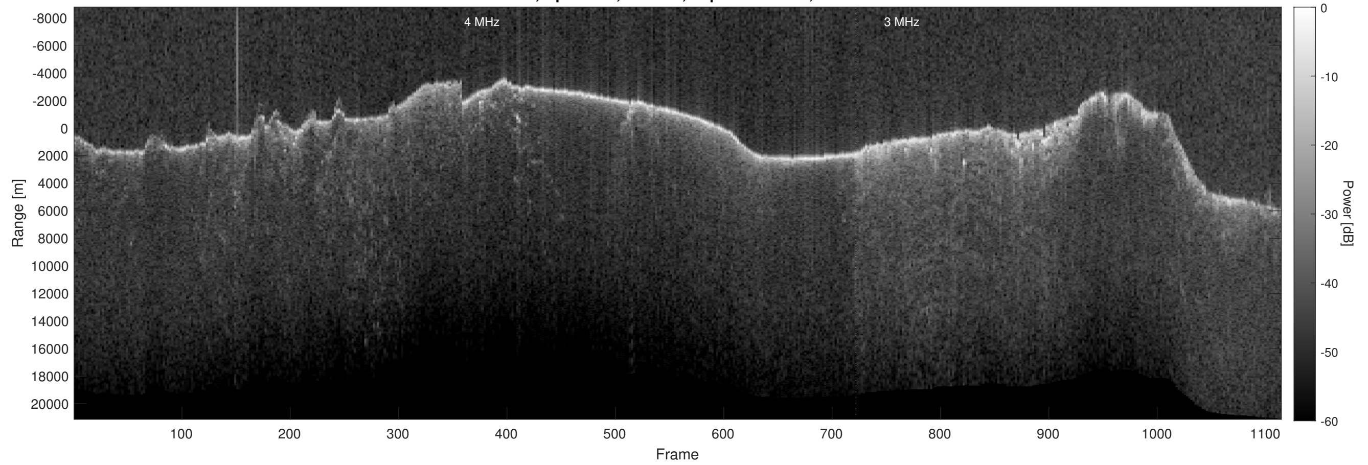
Orbit 4058, Optimized, Window, Depth-Corrected, Channel 2
