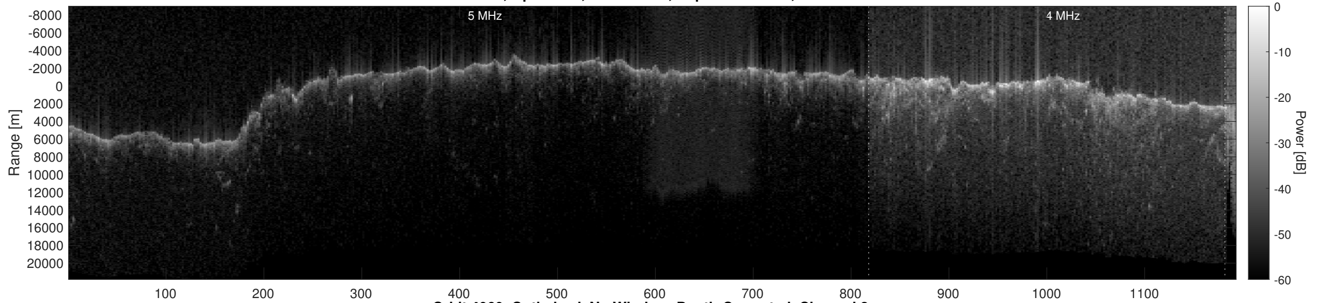
Orbit 4060, Optimized, No Window, Depth-Corrected, Channel 2
