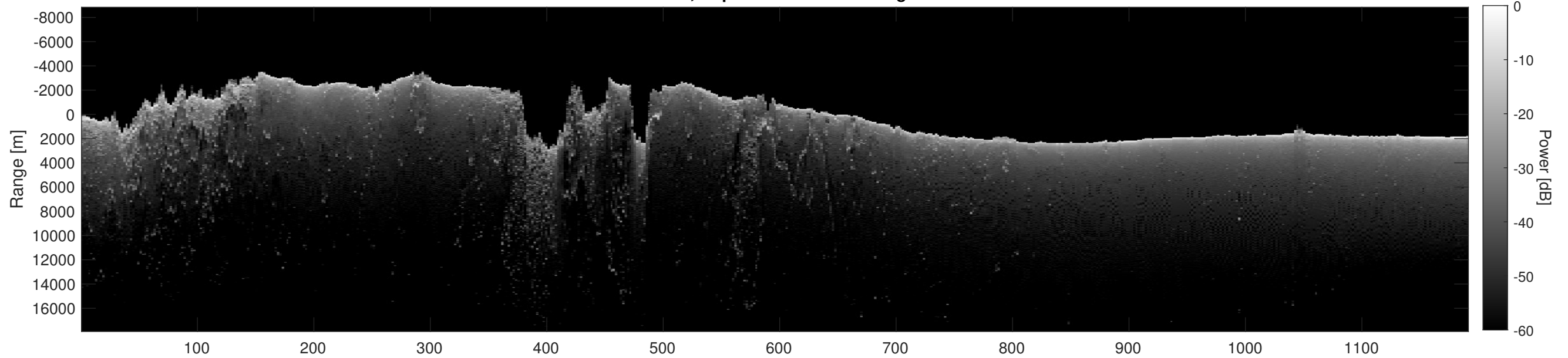
Orbit 4061, Depth-Corrected Cluttergram
