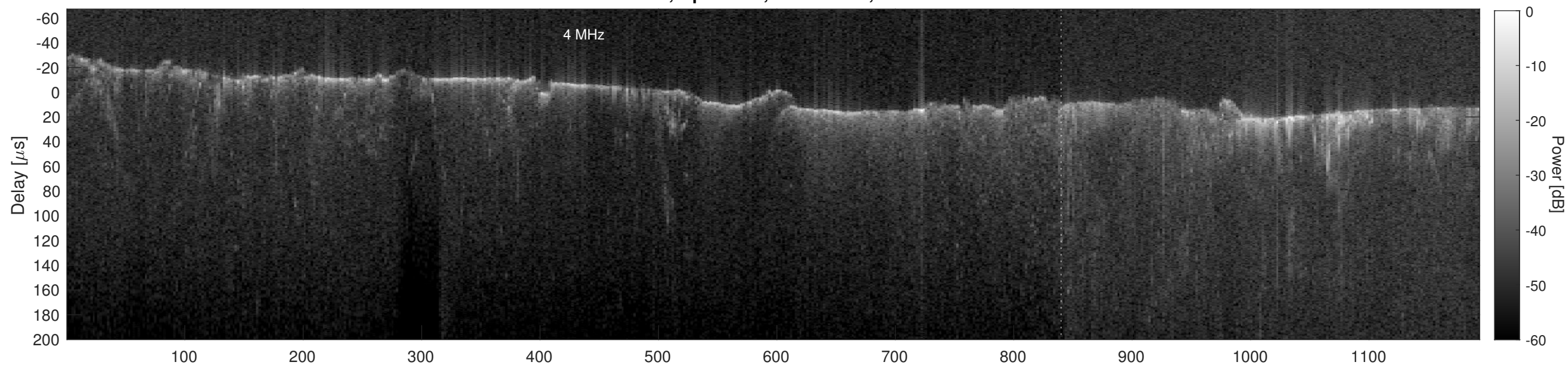
Orbit 4062, Cluttergram
