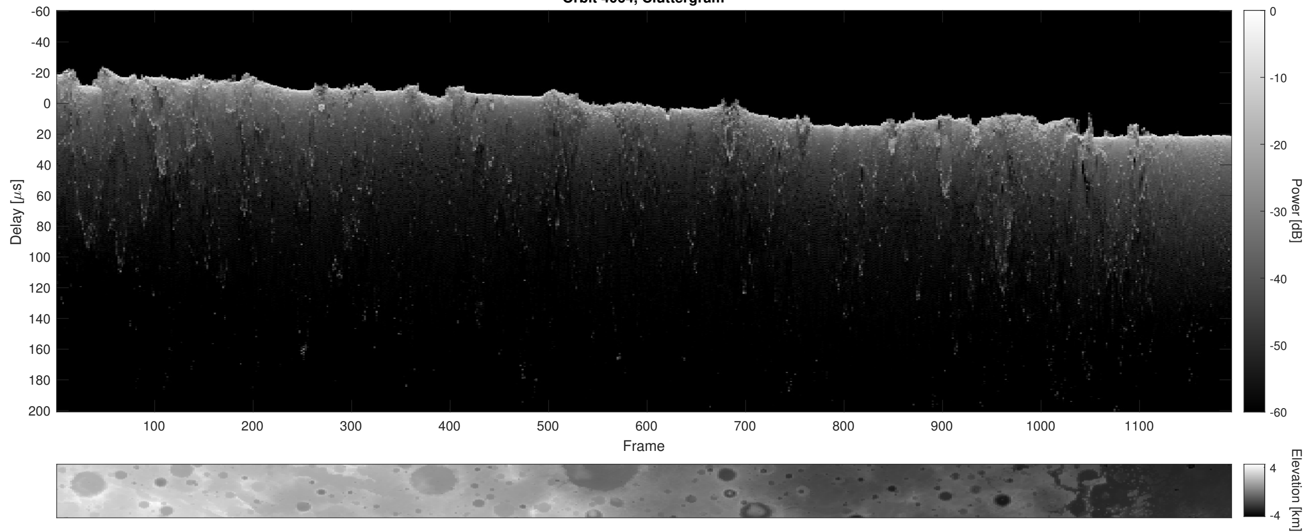
Orbit 4064, Cluttergram
