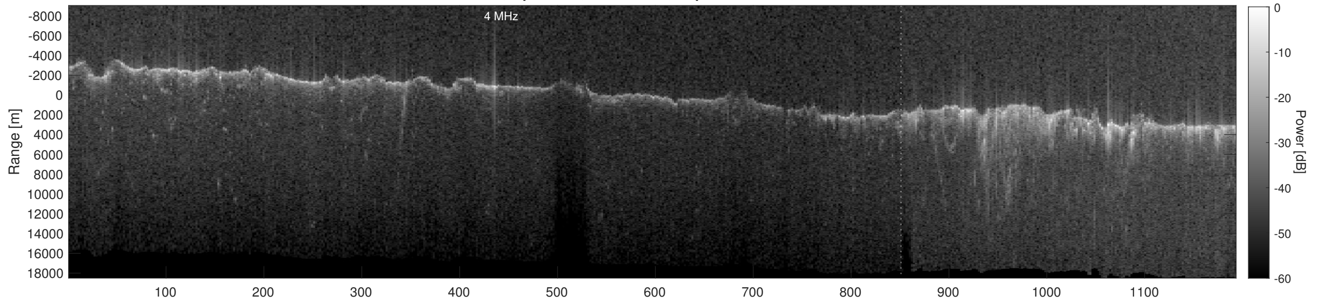
Orbit 4064, Depth-Corrected Cluttergram
