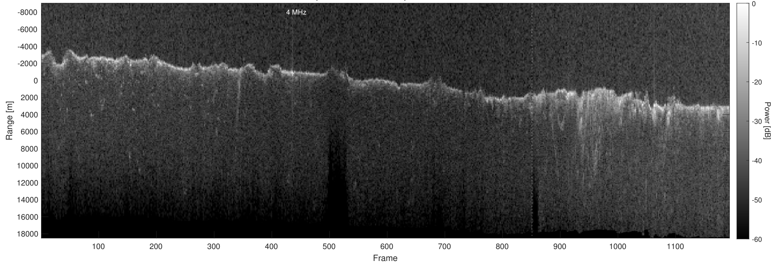
Orbit 4064, Optimized, Window, Depth-Corrected, Channel 2
