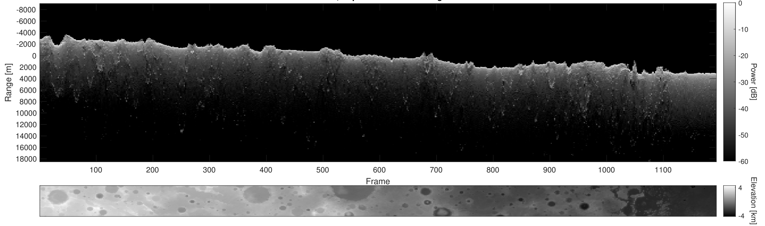
Orbit 4064, Depth-Corrected Cluttergram
