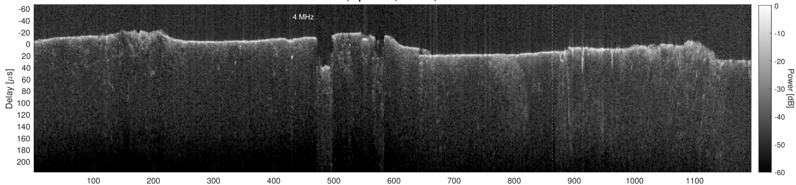
Orbit 4065, Cluttergram
