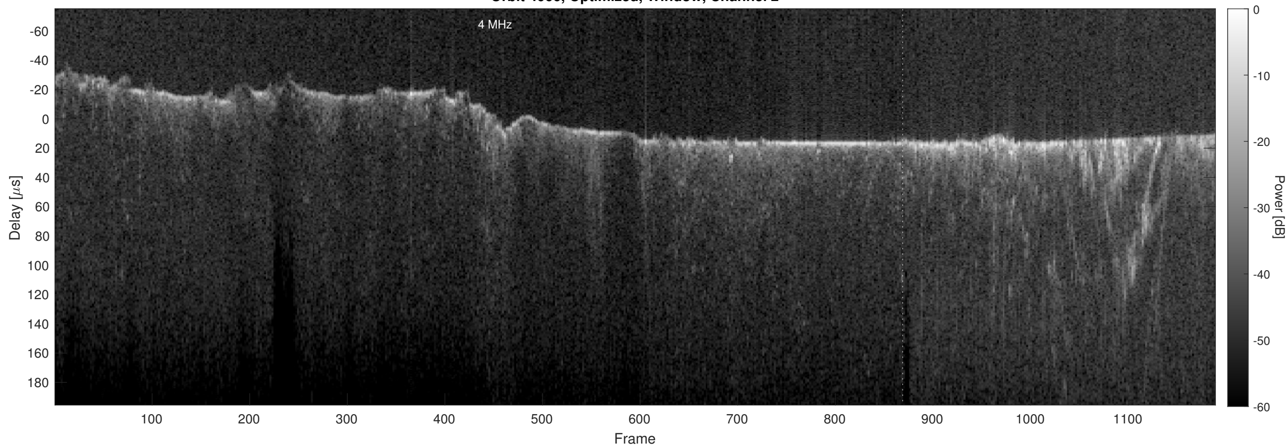
Orbit 4066, Optimized, Window, Channel 2
