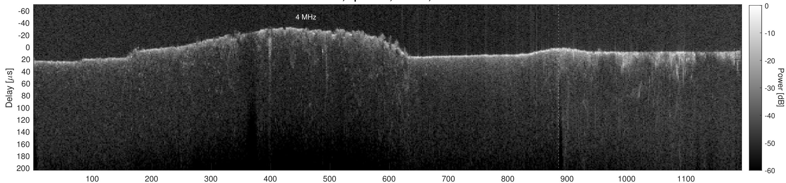
Orbit 4067, Cluttergram
