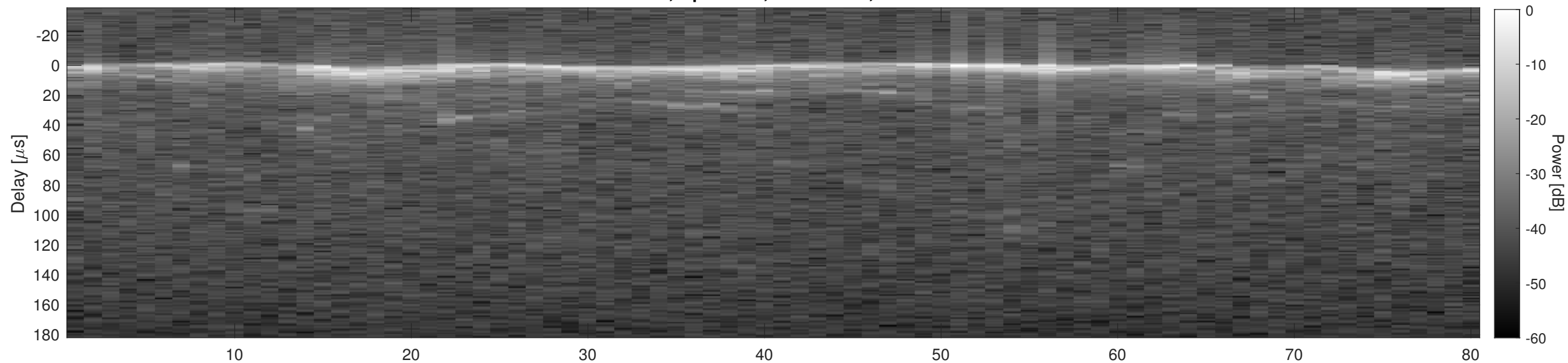
Orbit 4068, Cluttergram
