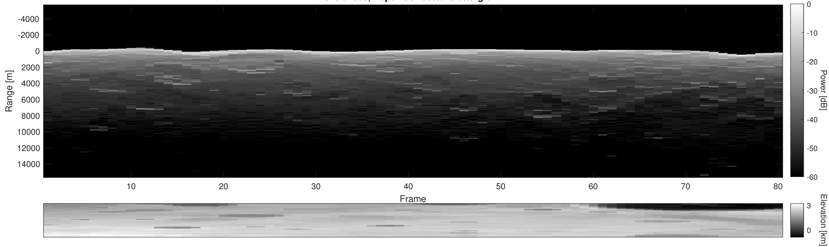
Orbit 4068, Depth-Corrected Cluttergram
