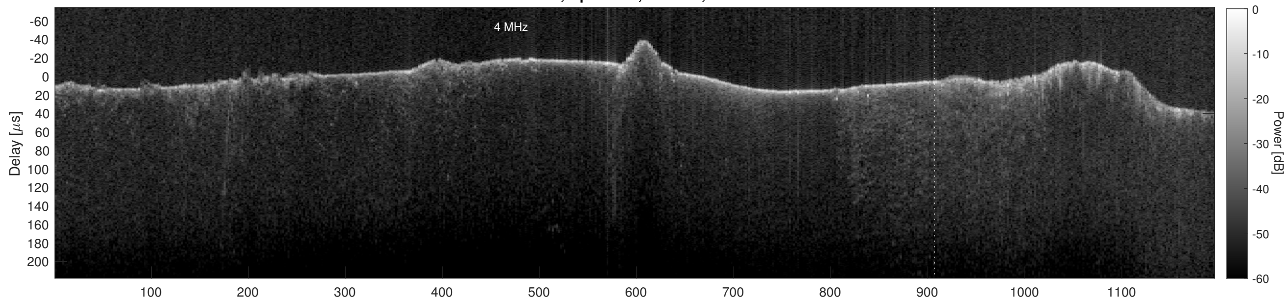
Orbit 4069, Cluttergram
