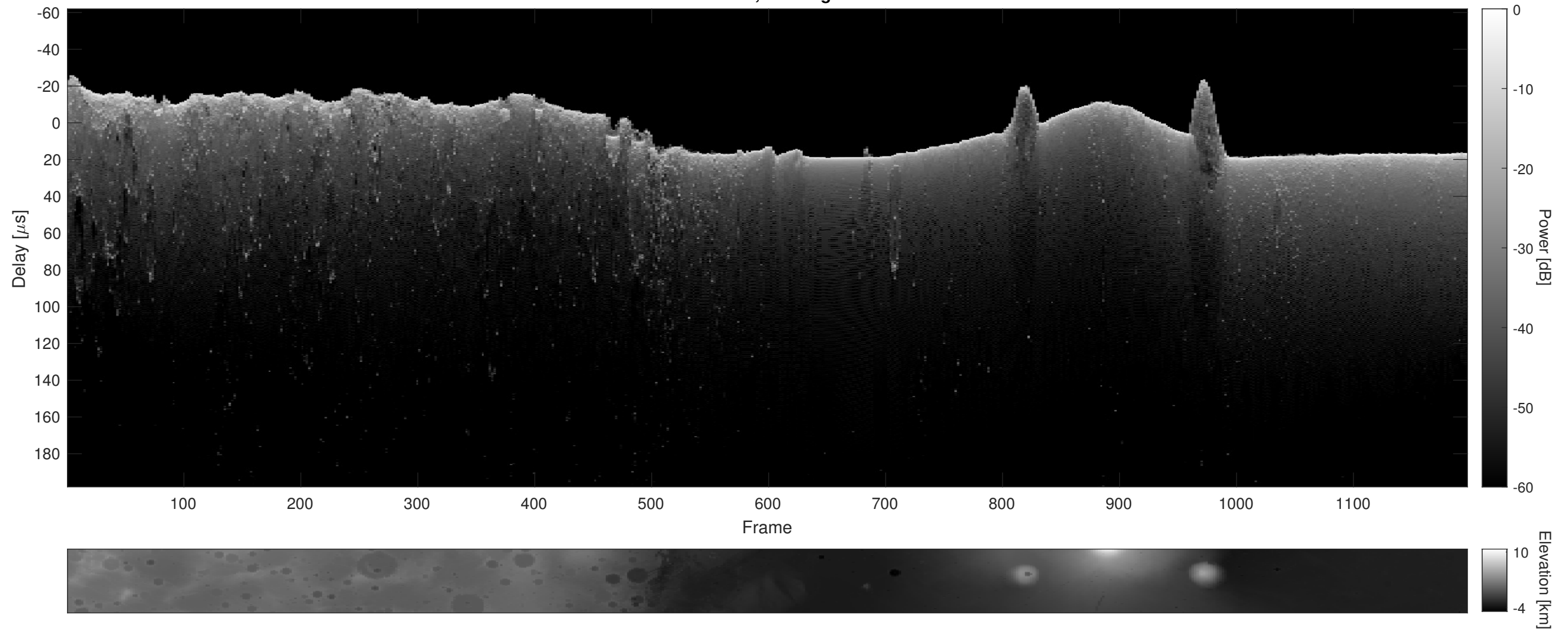
Orbit 4070, Cluttergram
