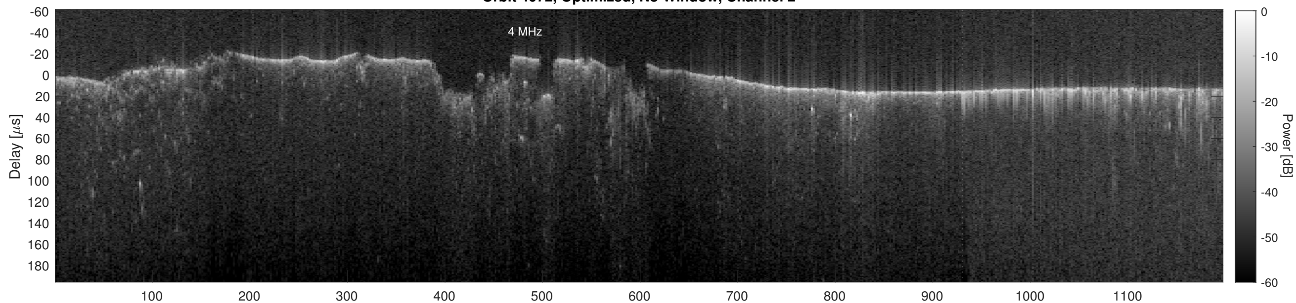
Orbit 4072, Cluttergram
