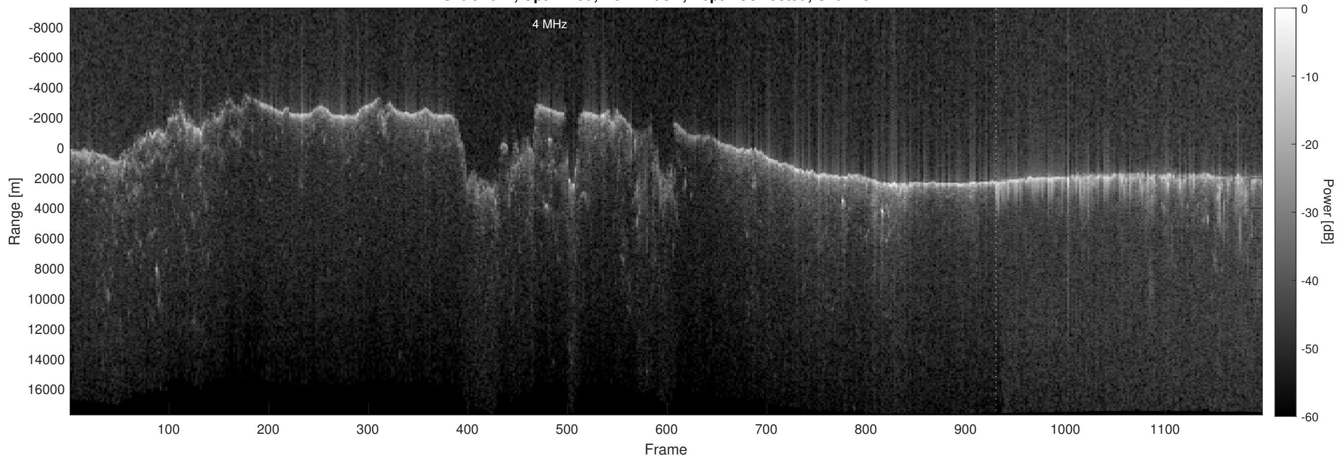
Orbit 4072, Optimized, No Window, Depth-Corrected, Channel 2
