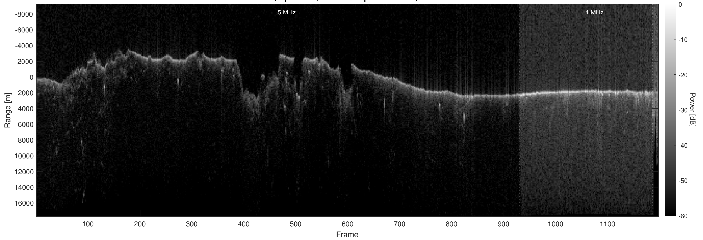
Orbit 4072, Optimized, Window, Depth-Corrected, Channel 2
