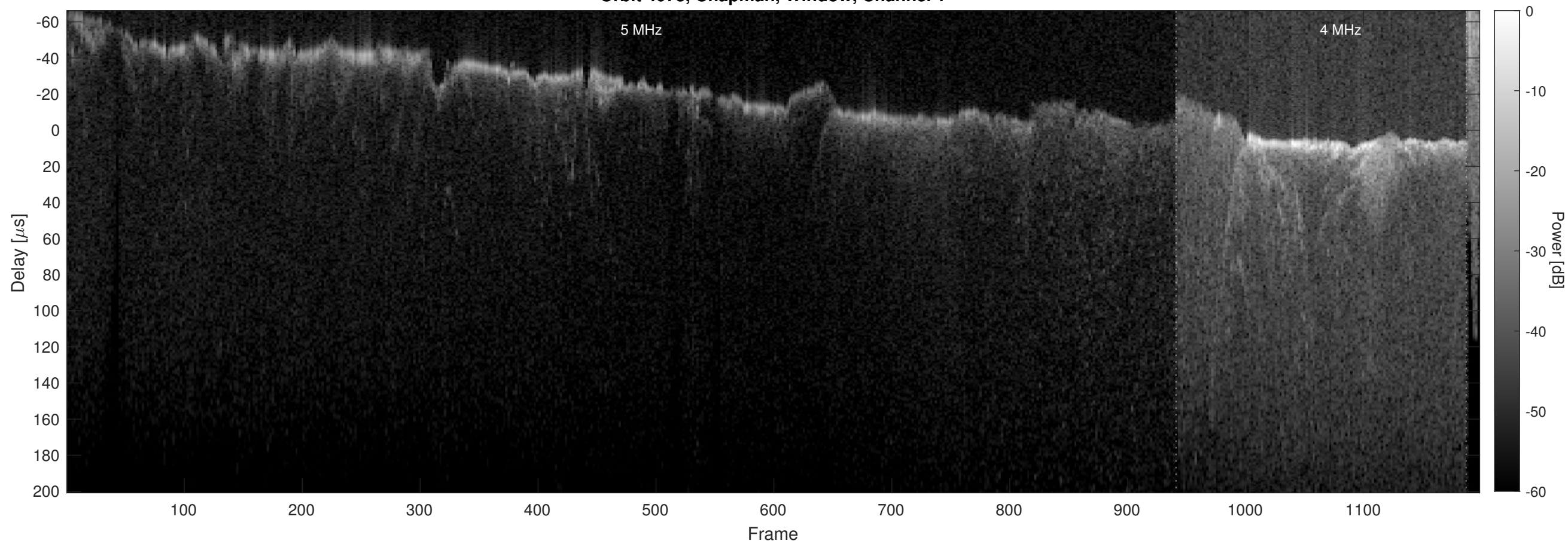
Orbit 4073, Chapman, Window, Channel 2
