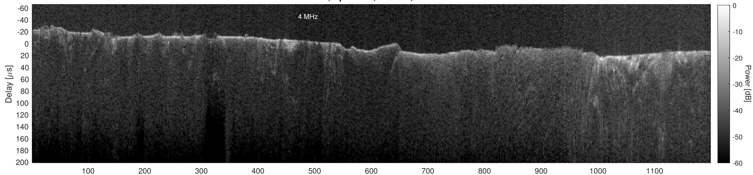
Orbit 4073, Cluttergram
