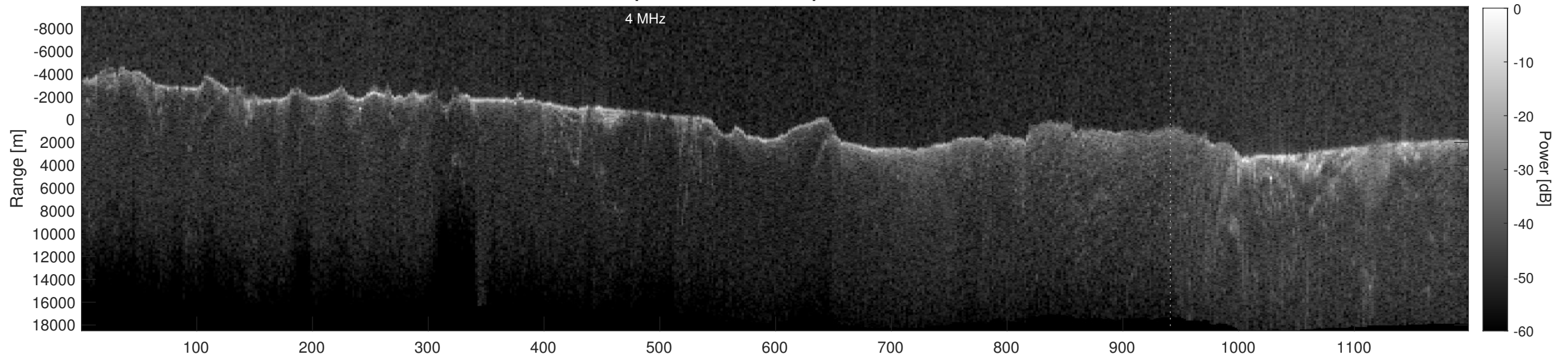
Orbit 4073, Depth-Corrected Cluttergram
