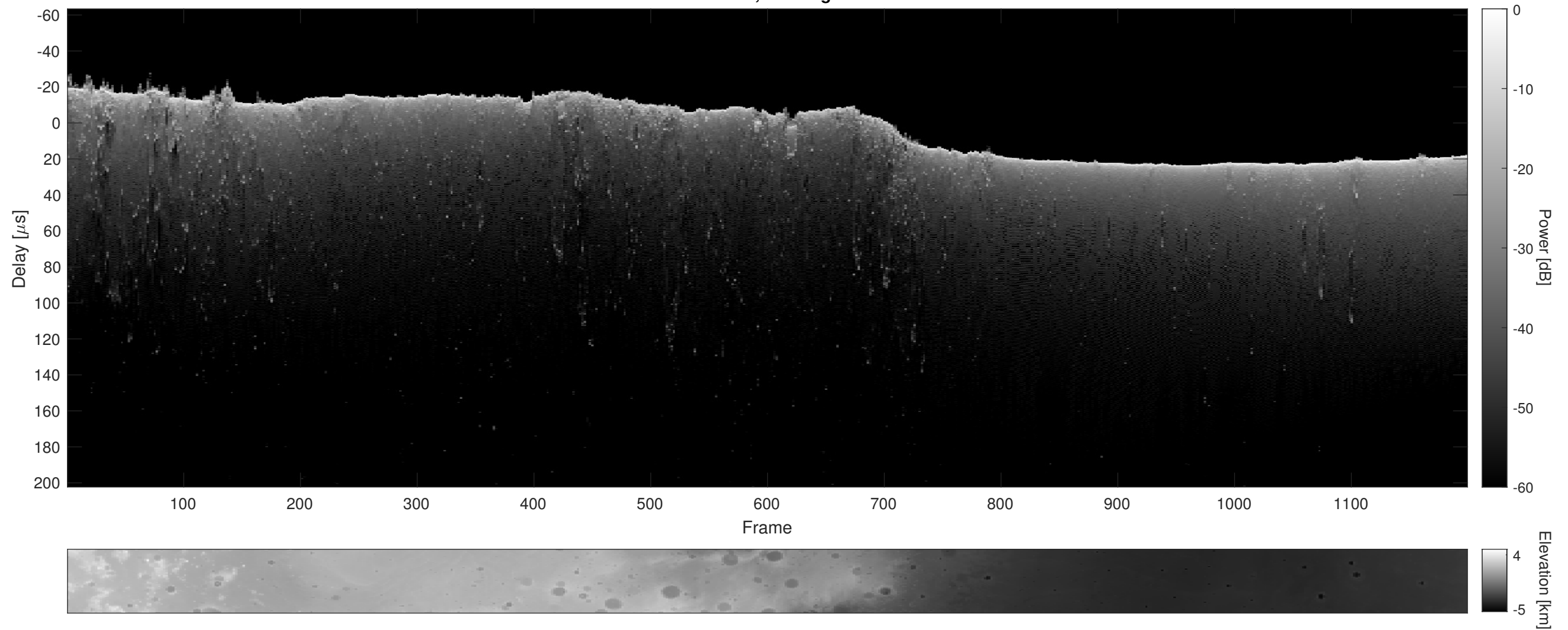
Orbit 4074, Cluttergram
