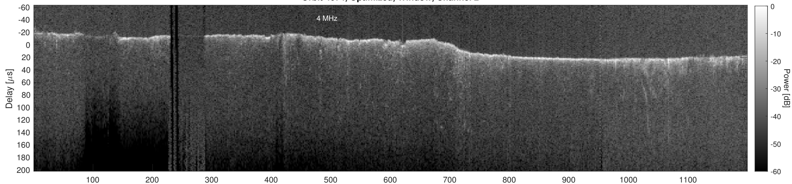
Orbit 4074, Cluttergram
