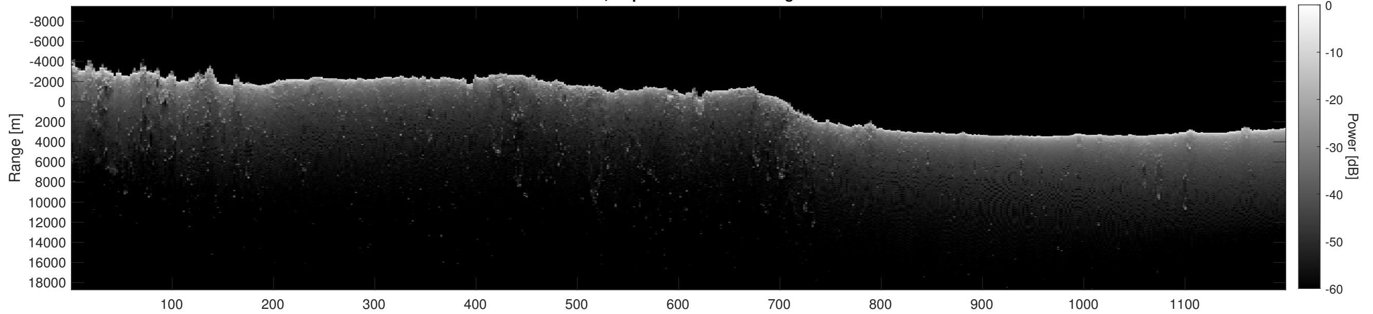
Orbit 4074, Depth-Corrected Cluttergram
