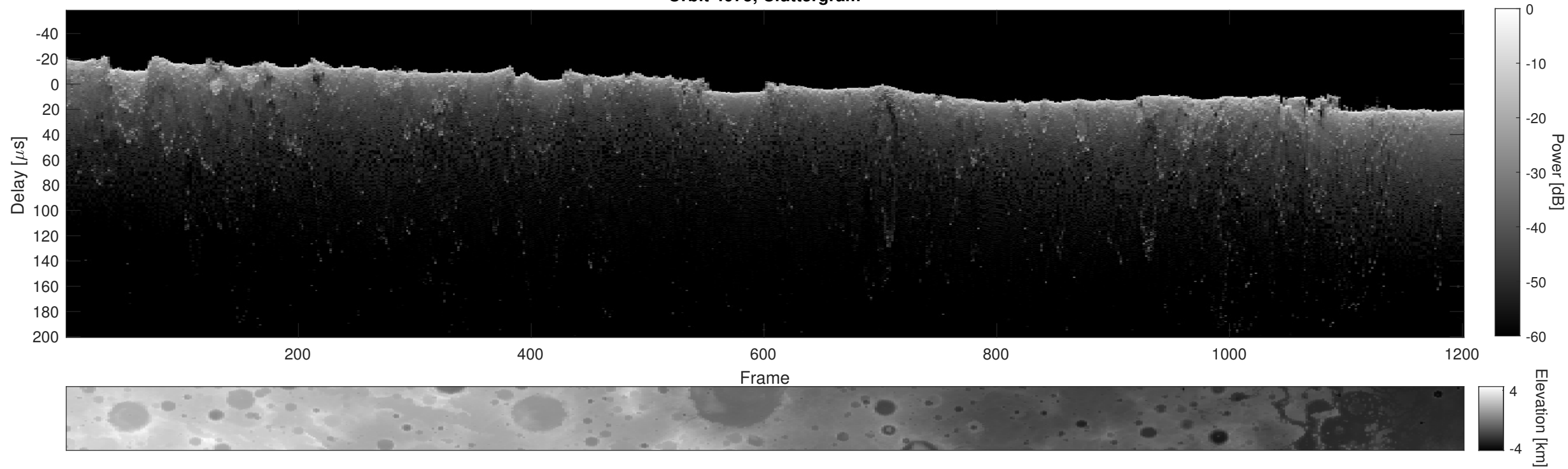
Orbit 4075, Cluttergram
