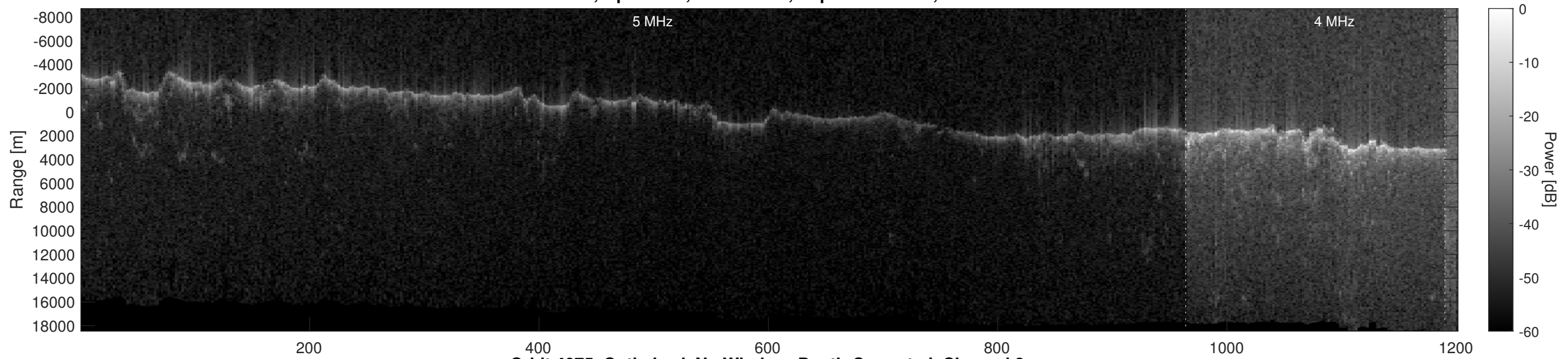
Orbit 4075, Optimized, No Window, Depth-Corrected, Channel 2
