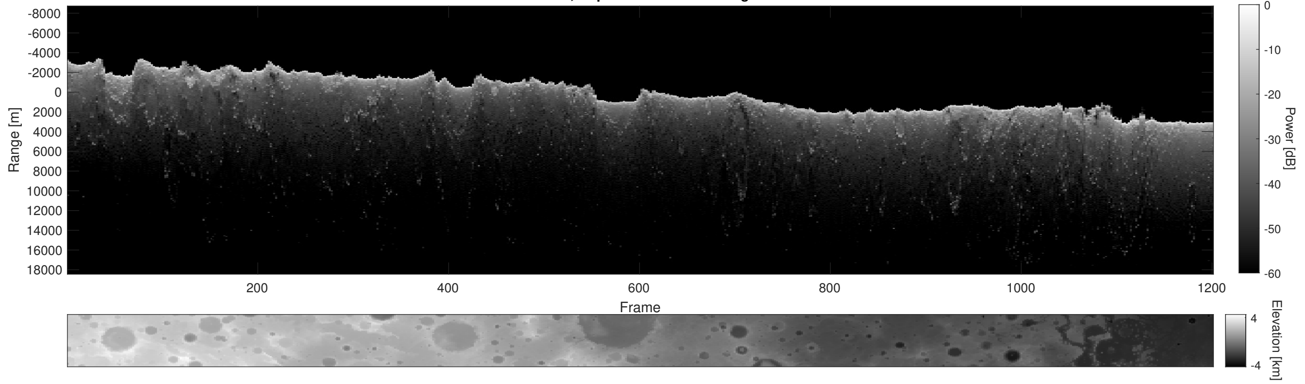
Orbit 4075, Depth-Corrected Cluttergram
