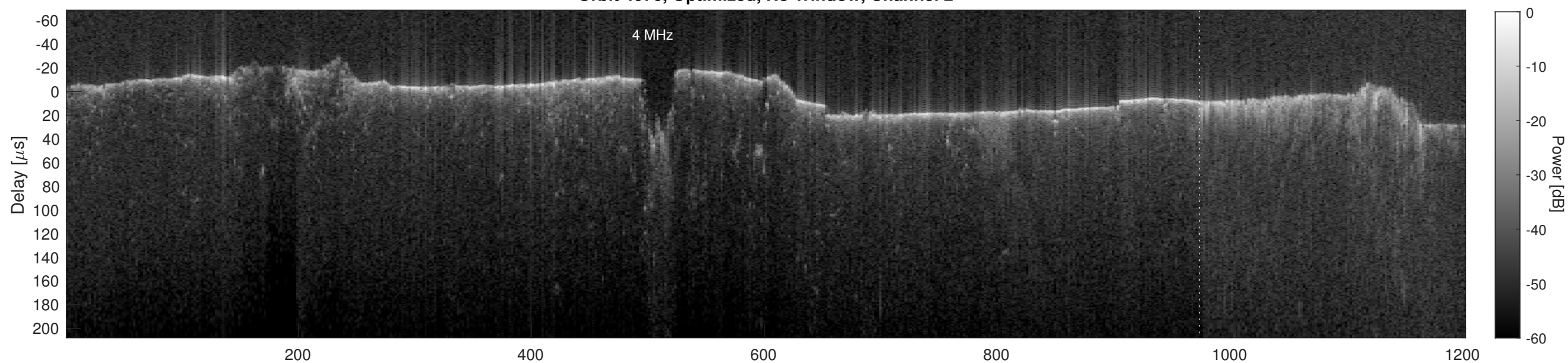
Orbit 4076, Cluttergram
